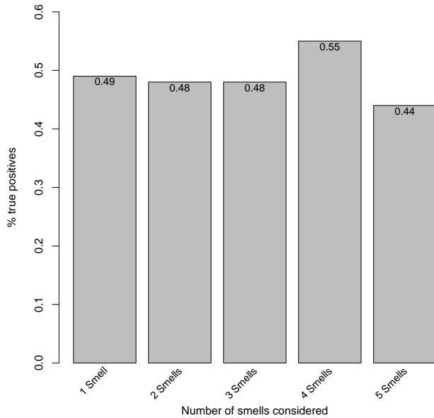
Fig. 6: Percentage of cells that contain errors from SFL's top 10% results.
