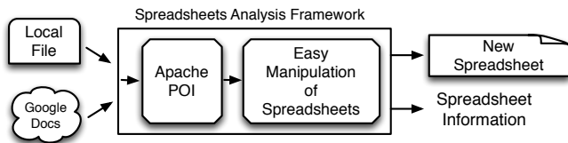
Fig. 2: The Spreadsheet Analysis Framework we used.
