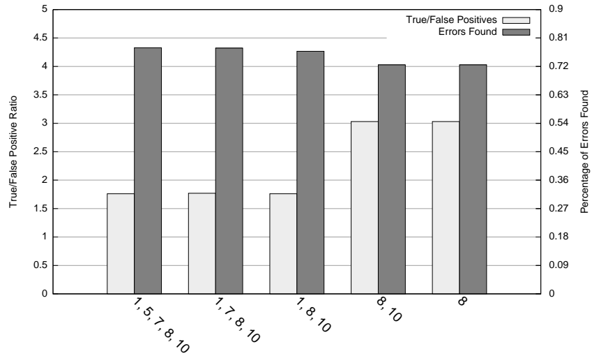
Fig. 5: Combination of 1 up to 5 of the smells with better results.
