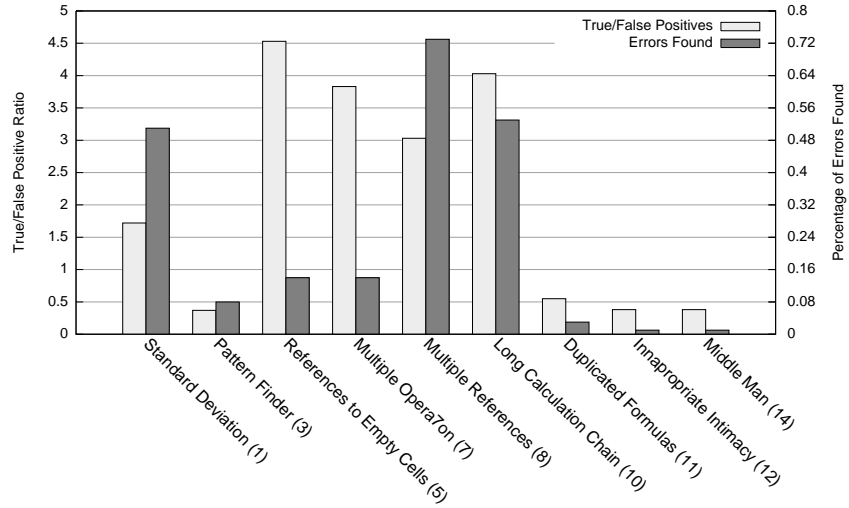
Fig. 4: True positive over false positives and percentage of errors found using single smells.
