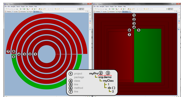
Figure 6: GZOLTAR visualizations comparative.
