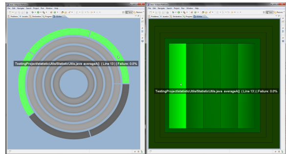
Figure 11: GZOLTAR root change.
